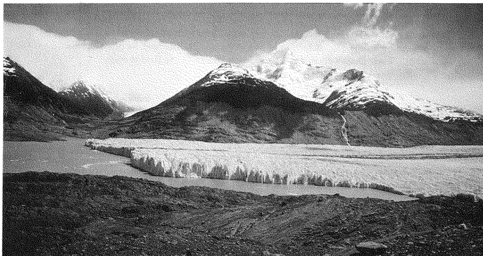
Fig. 8. Snout of Upsala Glacier in 1990 (Nov. 17), taken from the left bank. The northern end of islands can be seen on the left.
