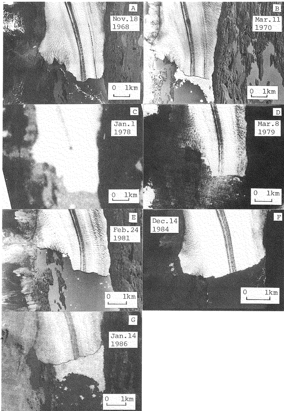
Fig. 6. Snout positions of Upsala Glacier in respective years. A, B, E, Argentine (IGM) photographs : C, Salyut-6 space photograph : D, Landsat RBV : F, Chilean (FACH) photograph : G, Landsat TM. Since these images are not rectified, scales are naturally approximate, and north is approximately top direction. As can be seen, islands are good reference features to compare the snout positions. In A and B, the same lump can be clearly recognized on the medial moraine, from which an average annual surface-flow velocity was derived.
