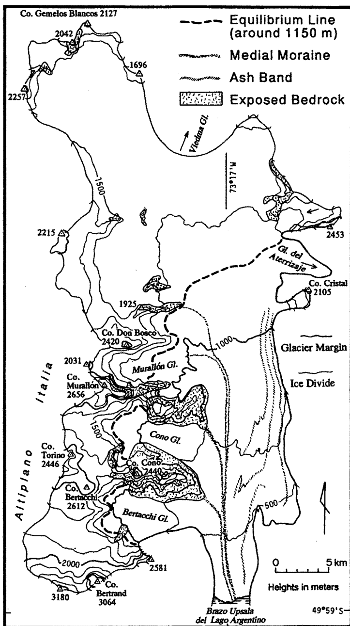
Fig. 2. The drainage area of Upsala Glacier (source : quadrangle Glaciar Viedma and Glaciar Upsala, both at a scale of 1 : 100,000). Co. (Cerro) means peak or mountain. The highest peak (3180 m) is listed as Co. Agassiz on the topographic map ; however, we believe that it is erroneously located. According to Lliboutry (1956) this is Co. Roma, and Co. Agassiz is given to a peak located due south. Co. Roma is renamed as Co. Vivod in 1969 by J. I. Skvarca after the first ascent. For these reasons we left out the name. Although the topographic maps do not differentiate medial moraines from ash bands, we indicated them separately because they could be easily identified on the aerial photographs. Ash layers are believed to have been deposited by eruptions of Volcan Lautaro, about 110 km to the north. Patterns of ash bands vary slightly on the aerial photographs of different dates.
