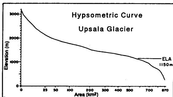
Fig. 3. The hypsometric curve of Upsala Glacier. The X axis is drawn on a scale of square root of the area so that the curve indicates a hypothetical profile of the drainage area when all the contours are drawn in concentric circles proportional to the respective areas. Since the slope of the curve around 1150 m (ELA) is gentle, a small shift of the ELA would cause a large change in the accumulation/ablation area.
